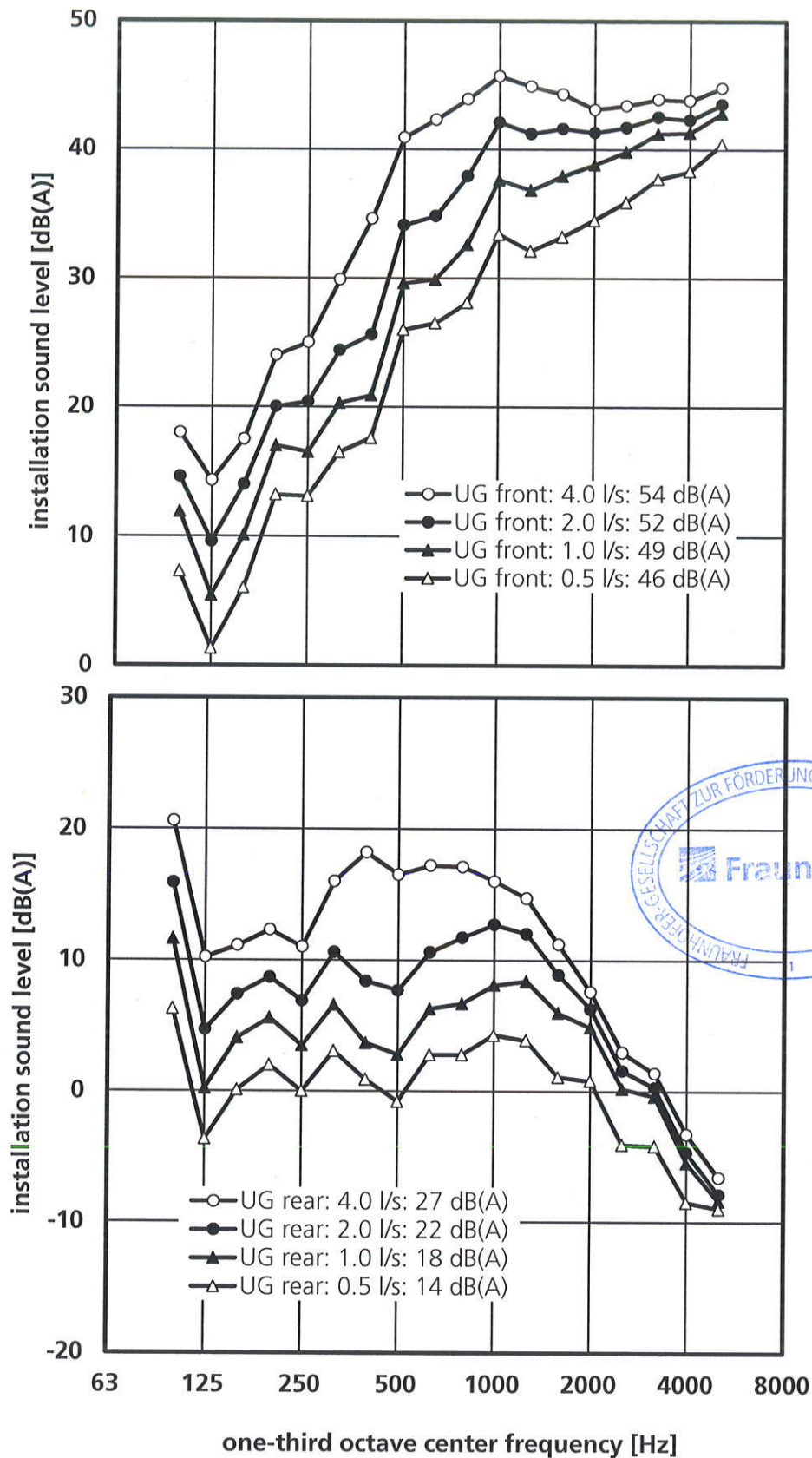
Figure 1 Wastewater installation system "ACO pipe" consisting of stainless steel pipes and fittings (manufacturer: ACO Industries k.s.) mounted with acoustic pipe clamps "Bismat 1000, one spacer" (manufacturer: Walraven) according to figure 4. The installation sound level L_{A\text{Feg},n} ( L_{In} ) according to DIN 4109 was measured at various flow rates in the test rooms UG front (above) and UG rear (below).
