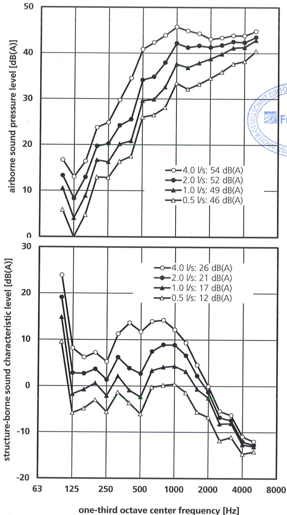
Figure 2 Wastewater installation system "ACO pipe" consisting of stainless steel pipes and fittings (manufacturer: ACO Industries k.s.) mounted with acoustic pipe clamps "Bismat 1000, one spacer" (manufacturer: Walraven) according to figure 4. Airborne sound pressure level L_{a,A} (above) and structure-borne sound characteristic level L_{sc,A} (below) measured at various flow rates according to EN 14366.
