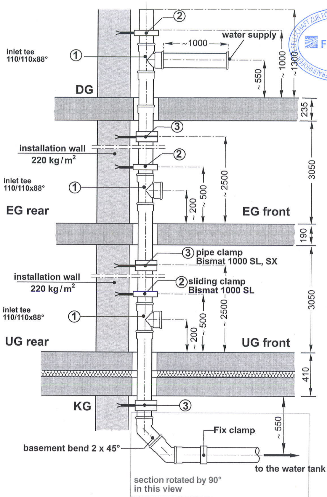
Figure 4 Installation plan of the wastewater installation system "ACO pipe" consisting of stainless steel pipes and fittings (manufacturer: ACO Industries k.s.) mounted with acoustic pipe clamps "Bismat 1000, one spacer" (manufacturer: Walraven). The guidance clamp (SL) and the sliding clamp (SL) were mounted with 7 mm space between the locking tabs of the clamp (one spacer on each side). Drawing not to scale, dimensions in mm.
